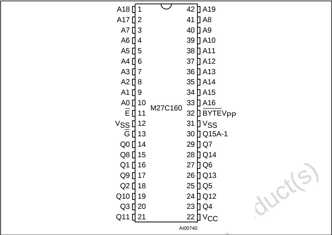
Figure 3. DIP Connections
