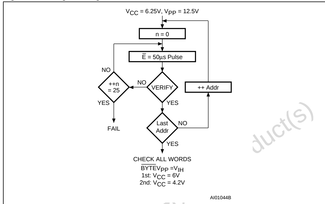
Figure 5. Programming Flowchart
